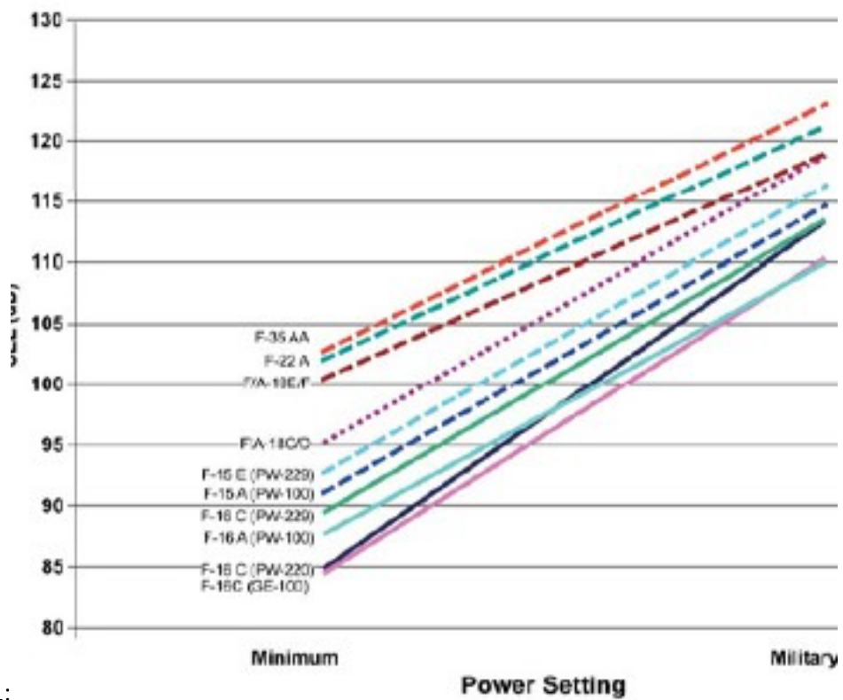
Normalized SEL vs. Aircraft Power Setting 1000' AGL Flyover Directly Under Flightpath
